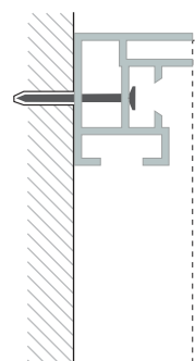
Drilling
